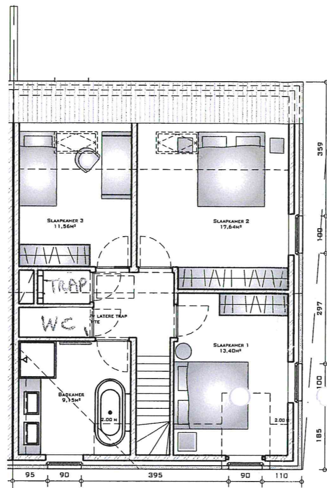
WONING LOT B VERDIEPING
